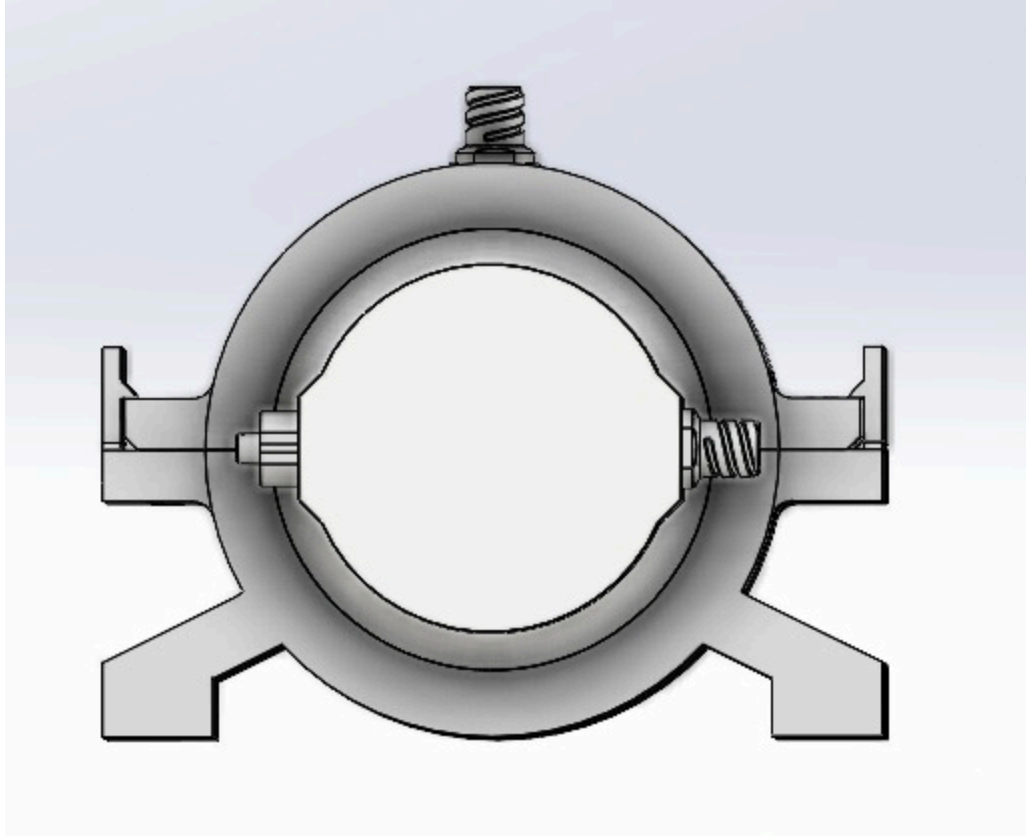
Latching mechanism close up (between two wrapping c-rings) (Overall num: 25)
